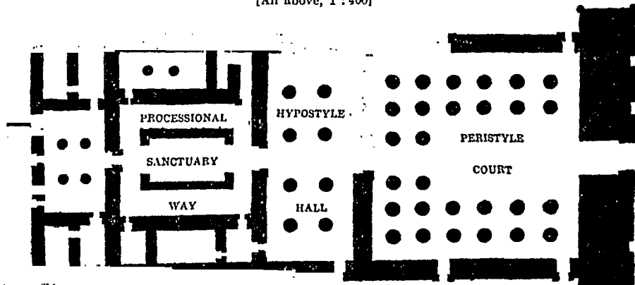
COMPLETE TEMPLE OF TWENTIETH DYNASTY. OF KHONSU, KARNAK
